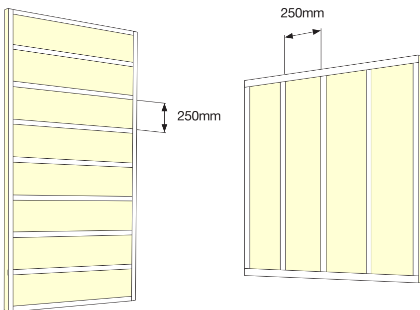
Examples of tape layout on sheet insulation showing how tape must be applied down each edge
